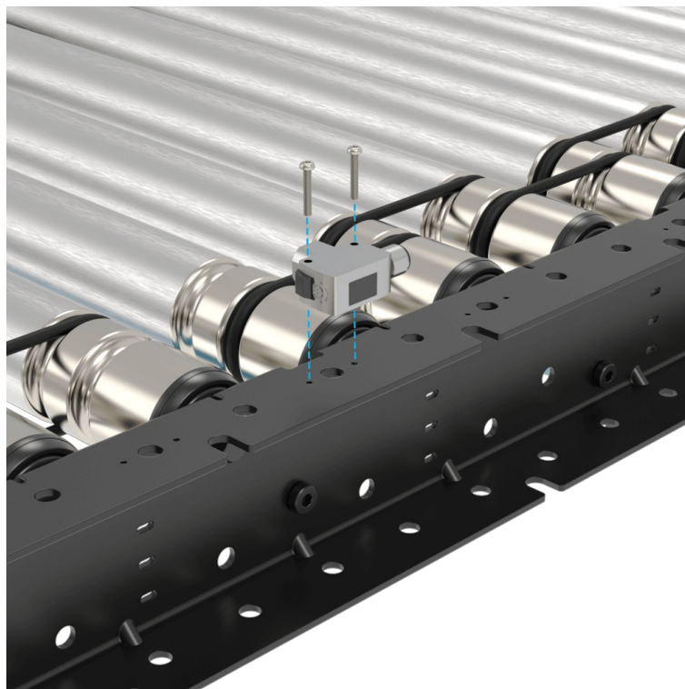
sensor installation
